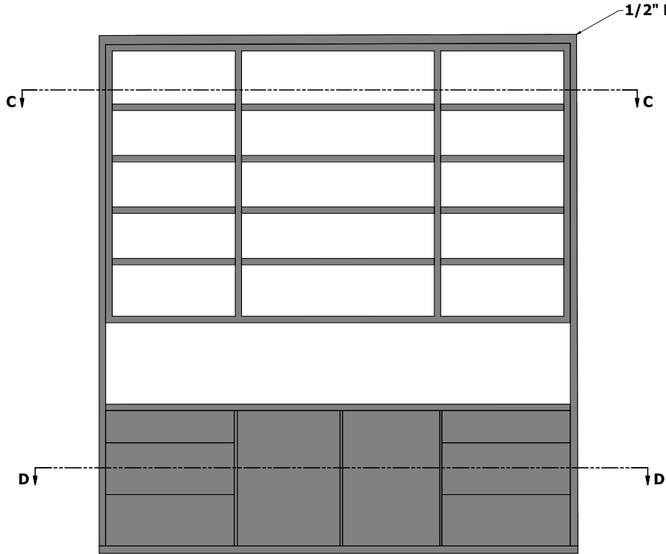
Front View SCALE 0.03 : 0.3
